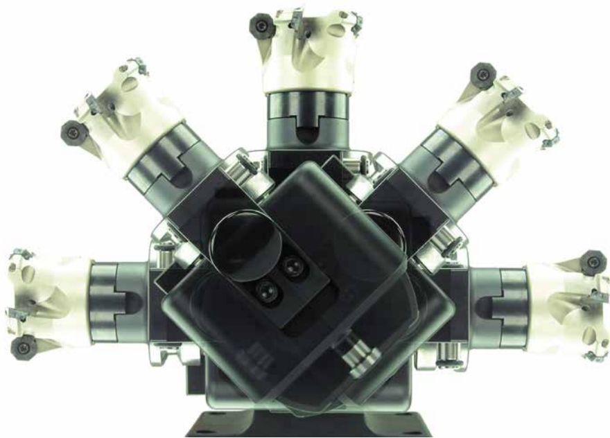
200090 alfa-clamp 90
